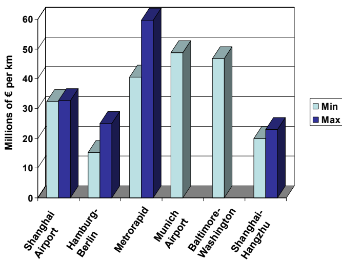
Figure 3: Comparison of Estimated Building Costs per Kilometre
