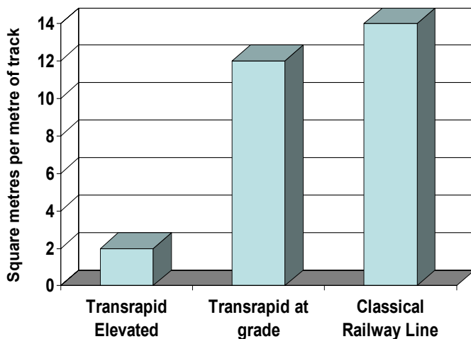
Figure 1: Land Use for the Transrapid System Compared to Conventional Railway
